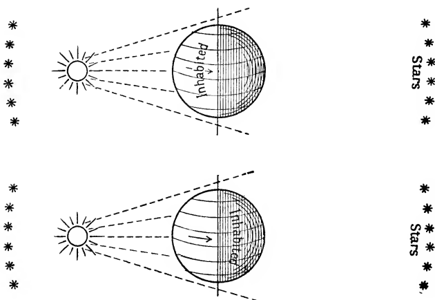
Fig. 18. Earth and sun according to Heracleides.
